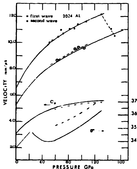
Figure 6. Wave velocities as a function of pressure. The dots and circles are velocities calculated from the experiment data. The shear velocity, C_v , and Poisson's ratio, \sigma , were calculated from the upper sets of curves.
